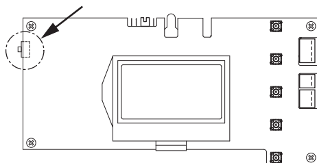
RJ12 connector for remote start module
